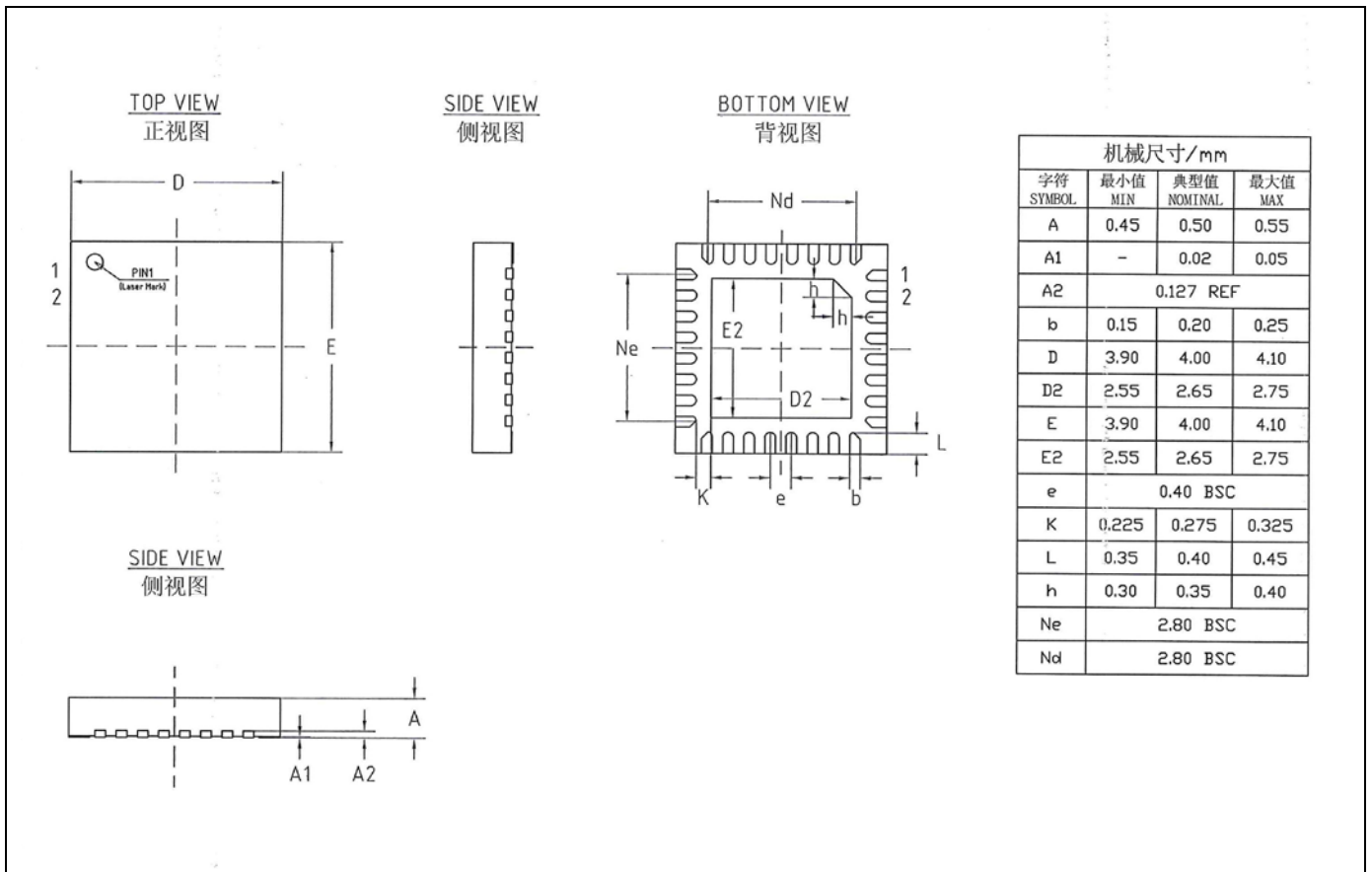
Figure 4-5 32-QFN (4x4-P0.4mm)封装尺寸
