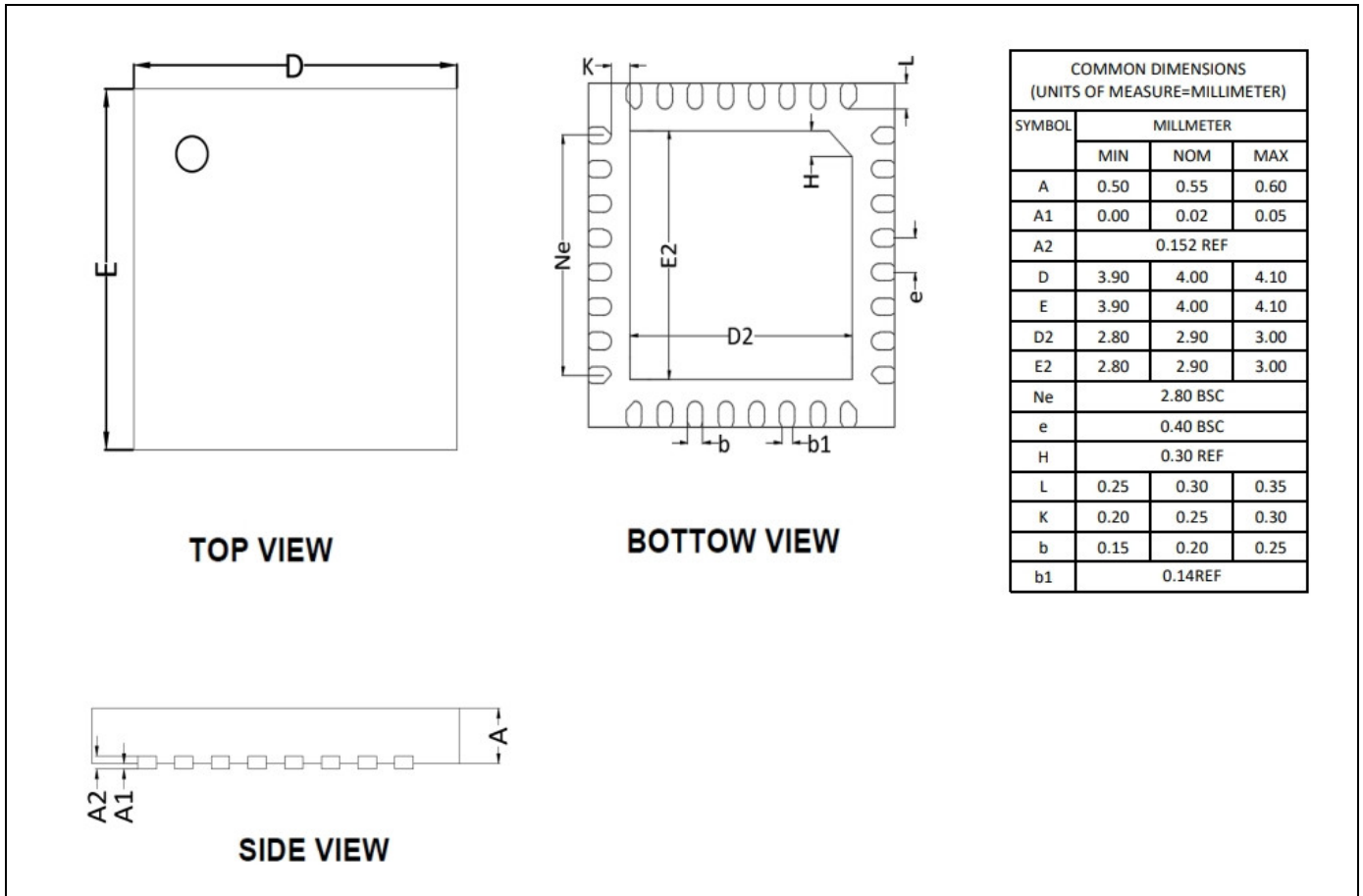
Figure 4-4 32-QFN (4x4-P0.4mm)封装尺寸
