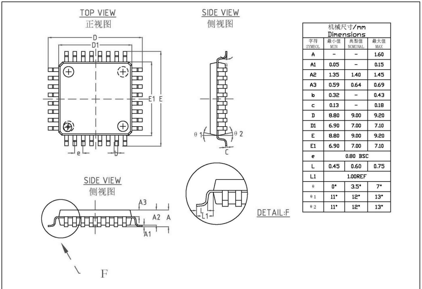
Figure 4-1 32-LQFP封装尺寸
