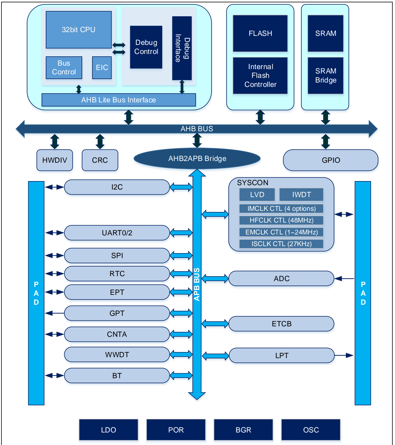
Figure 1-1 APT32S003F7P6模块框图
